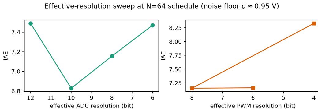
FIGURE 9. Effective-resolution sweep at the N=64 achievable schedule. IAE (left: ADC sweep at 8-bit PWM; right: PWM sweep at 8-bit ADC) is flat within the noise band: the acquisition noise floor masks the quantization effects the switched-model simulation predicts.
