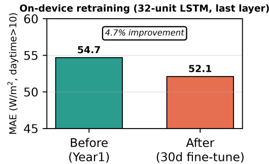
Figure 21. On-device retraining on ESP32-S3 N16R8 (8 MB PSRAM): 30-day 720-sample ring buffer, 5 epochs at 1e-4 , last-layer only (33 params). MAE 54.68 to 52.10 \text{W/m}^2 (4.7% improvement) on Year-2 hold-out. Model 17 kB, ring buffer 2.9 kB, 766 ms total.
