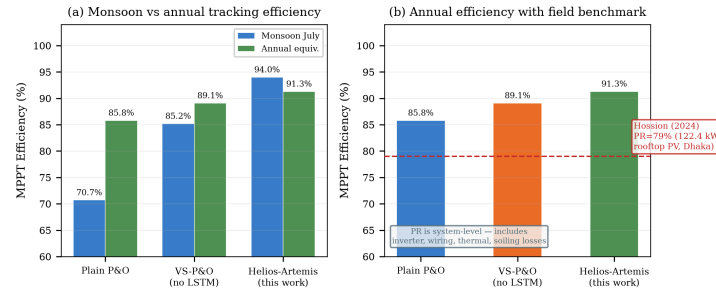
Figure 8. Simulated MPPT efficiency comparison. (a) Monsoon vs annual tracking efficiency for three controller types. (b) Annual efficiency with Hosson [22] system-level PR reference (79%, 122.4 kW rooftop PV, Dhaka). PR includes all system losses and is not directly comparable to MPPT tracking efficiency.
