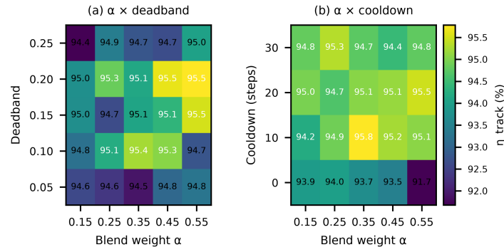
Figure 14. Multidimensional sensitivity of the LSTM-P&O tracking efficiency on the stochastic day (seed 23, 1 h, \text{dt} = 0.1 s): (a) \alpha \times deadband, (b) \alpha \times cooldown, all other factors at baseline. The \alpha \in [0.25, 0.45] , deadband \in [10\%, 20\%] plateau varies by less than 1 pp about 95.1%.
