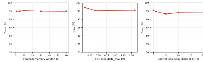
Figure 15. One-dimensional sensitivity of LSTM-P&O tracking efficiency on the stochastic day (seed 23, \text{dt} = 0.1 s): (a) forecast-memory window, (b) variable-step P&O size delta_max, (c) control-loop (UART) latency in 0.1 s ticks. Baselines: 10 s window, 0.80 V, zero delay.
