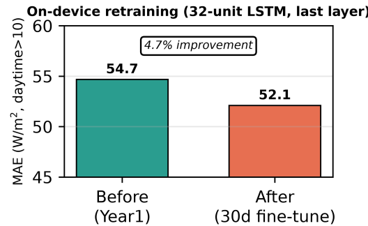
Figure 21. On-device retraining on ESP32-S3 N16R8 (8 MB PSRAM): 30-day 720-sample ring buffer, 5 epochs at 1e-4 , last-layer only (33 params). MAE 54.68 to 52.10 W/m^2 (4.7% improvement) on Year-2 hold-out. Model 17 kB, ring buffer 2.9 kB, 766 ms total.
