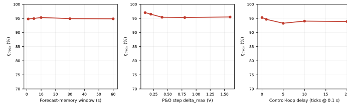
Figure 15. One-dimensional sensitivity of LSTM-P&O tracking efficiency on the stochastic day (seed 23, dt = 0.1 s): (a) forecast-memory window, (b) variable-step P&O size \Delta_{\text{max}} , (c) control-loop (UART) latency in 0.1 s ticks. Baselines: 10 s window, 0.80 V, zero delay.
