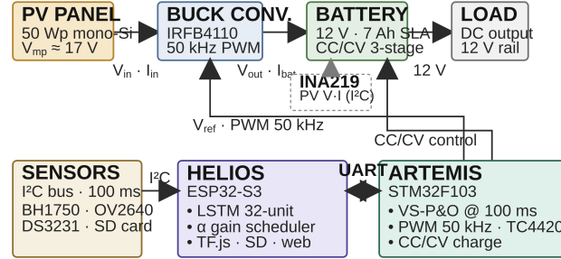
Figure 1. Helios-Artemis dual-MCU predictive MPPT system architecture. Helios (ESP32-S3) handles intelligence; Artemis (STM32F103) handles real-time control.
