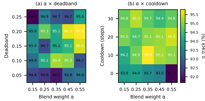
Figure 14. Multidimensional sensitivity of the LSTM-P&O tracking efficiency on the stochastic day (seed 23, 1 h, dt = 0.1 s): (a) \alpha \times deadband, (b) \alpha \times cooldown, all other factors at baseline. The \alpha \in [0.25, 0.45] , deadband \in [10\%, 20\%] plateau varies by less than 1 pp about 95.1%.
