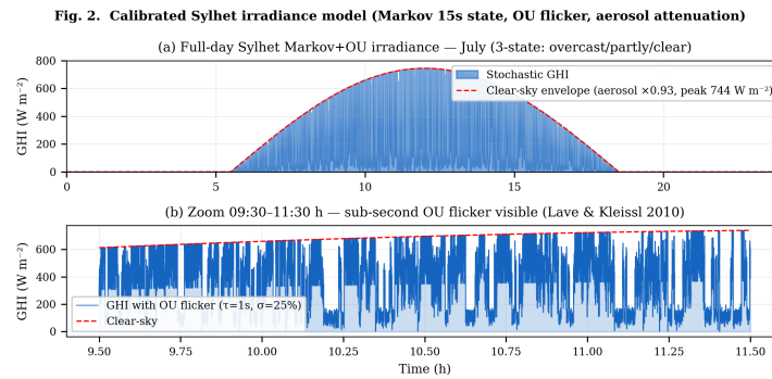
Figure 2. Calibrated Sylhet Markov-chain + Ornstein-Uhlenbeck (Markov+OU) irradiance model (July). (a) Full-day profile. (b) Zoom 09:30–11:30 h showing sub-second OU flicker.
