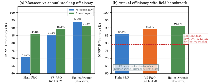
Figure 8. Simulated MPPT efficiency comparison. (a) Monsoon vs annual tracking efficiency for three controller types. (b) Annual efficiency with Hossion [22] system-level PR reference (79%, 122.4 kW rooftop PV, Dhaka). PR includes all system losses and is not directly comparable to MPPT tracking efficiency.
