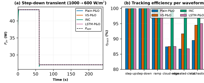
Figure 16. Controlled transient benchmark across all four controllers under identical conditions: (a) post-step power traces on the step-down waveform against the analytic P_{MPP} , (b) tracking efficiency per waveform (pattern-coded). Values are summarised in Table 4.
