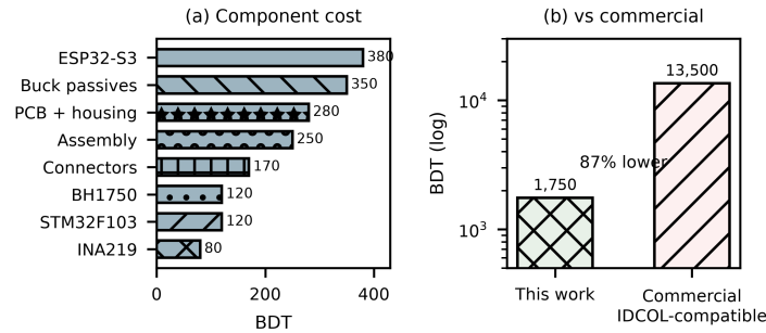
Figure 20. BOM breakdown and cost comparison. Total 1,750 BDT — 87% below IDCOL-compatible commercial MPPT (Dhaka retail, Q1 2026).
