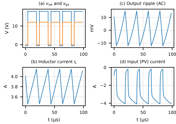
Figure 11. Buck power-stage switching waveforms at the nominal 3.8 A operating point (ngspice, 20 ns timestep): (a) switch node and gate–source voltage, (b) inductor current (CCM), (c) output voltage ripple, (d) PV input current.
