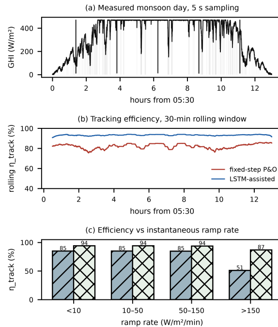
Figure 13. Efficiency evidence on a measured monsoon day (17 Aug 2026, 5 s sampling): (a) irradiance trace with the highest-variability 20% of windows shaded; (b) day-long energy-weighted tracking efficiency, fixed-step P&O vs LSTM-assisted; (c) tracking efficiency stratified by instantaneous ramp rate.
