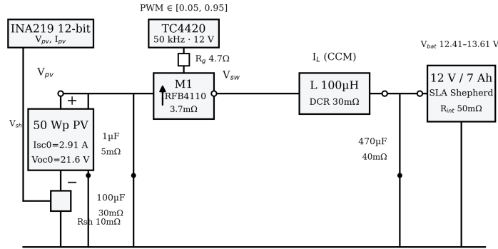
Figure 10. Power-stage schematic with signal names and measurement points ( V_{pv} , I_{pv} via INA219 shunt, v_{gs} , v_{sw} , i_L , v_{bat} ): 50 Wp PV panel, IRFB4110 with freewheeling body diode, TC4420 gate driver (50 kHz, 12 V, R_g = 4.7 \text{ }\Omega ), LC filter ( L = 100 \text{ }\mu\text{H} , DCR 30 \text{ m}\Omega ; C = 470 \text{ }\mu\text{F} , ESR 40 \text{ m}\Omega ), 12 V/7 Ah SLA battery ( R_{int} = 50 \text{ m}\Omega ).
