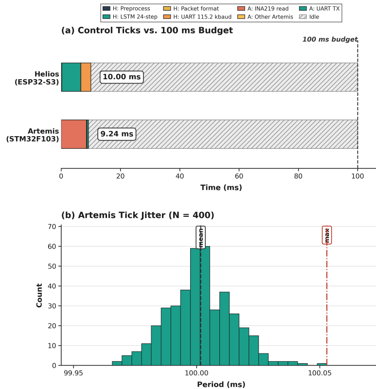
Figure 18. Measured dual-MCU execution-time budget ( N = 400 each): (a) Helios (ESP32-S3, 240 MHz, serial monitor) and Artemis (STM32F103C8T6, 72 MHz, DWT_CYCCNT direct FTDI) control ticks against the 100 ms budget (Artemis 9.24 ms, Helios 10.00 ms, \sim 90 ms idle); (b) Artemis 100 ms loop-period distribution (mean 100.00 ms, p99 100.06 ms, max 100.06 ms). The 3.58 ms Helios-UART \rightarrow Artemis-PWM path is an order of magnitude below the 5 s cloud-edge transient.
