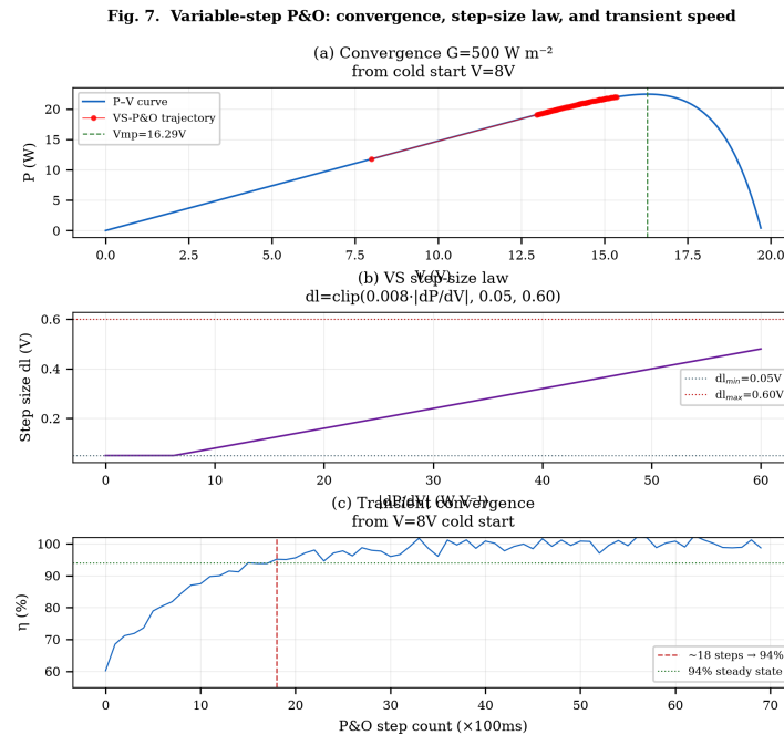
Figure 7. VS-P&O: (a) convergence trajectory on P–V curve, (b) step-size law, (c) transient convergence speed ( \sim 18 steps to 94% from cold start).
