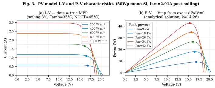
Figure 3. PV model I–V and P–V characteristics (50 Wp mono-Si, I_{sc0} = 2.91 A post-soiling, k = 14.26 ). Dots mark true MPP from exact analytical solution.
