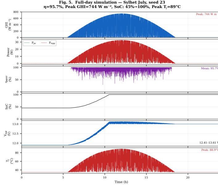
Figure 5. Full-day simulation results — Sylhet July (seed 23). Six panels: GHI, P_{pv} vs P_{mpp} , \eta_{MPPT} , SoC, V_{bat} , T_J .
