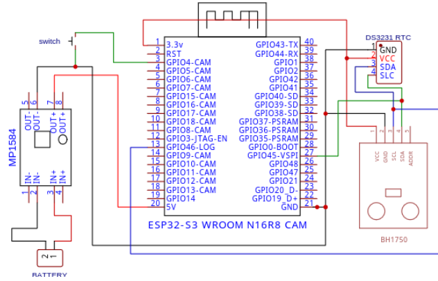
Figure 17. Field logger schematic: ESP32-S3 WROOM N16R8 CAM, GY-302 BH1750 light sensor, DS3231 RTC, MP1584 buck converter (12 V input \rightarrow 3.3 V/5 V rails), and battery/switch interfaces (Leading University, REV 1.0).
