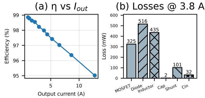
Figure 12. (a) Converter efficiency versus output current (98.9% at 1.0 A to 95.0% at 12.8 A; 98.0% at the 3.8 A point). (b) Loss breakdown at 3.8 A: MOSFET 0.32 W, body diode 0.52 W, inductor DCR 0.43 W, shunt 0.10 W, capacitor ESR 0.03 W (total 1.41 W).
