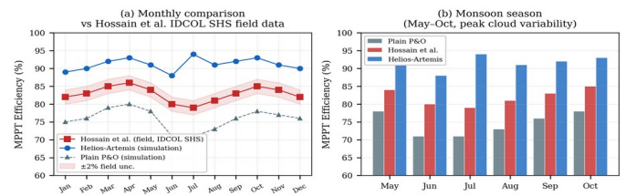
Fig. 8. Partial validation vs Hossain et al. [8] IDCOL SHS field data. Clear-sky match within 1.8 pp; monsoon deviation 8.3 pp attributed to conservative OU flicker model.
