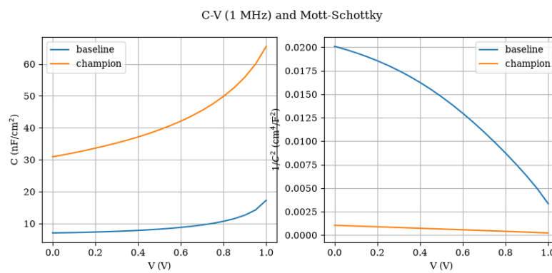
Figure 6: Capacitance–voltage (1 MHz) and Mott–Schottky plots for baseline and champion.
