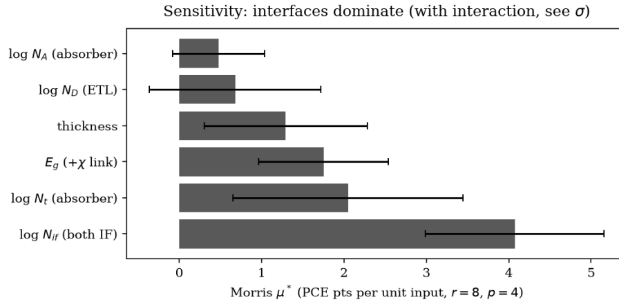
Figure 11: Morris \mu^* (bars) with interaction spread \sigma (whiskers). Ranking is regime-conditional: interfaces lead at the defect floor, bulk defects at routine levels (Table 12); large \sigma signals interactions.
