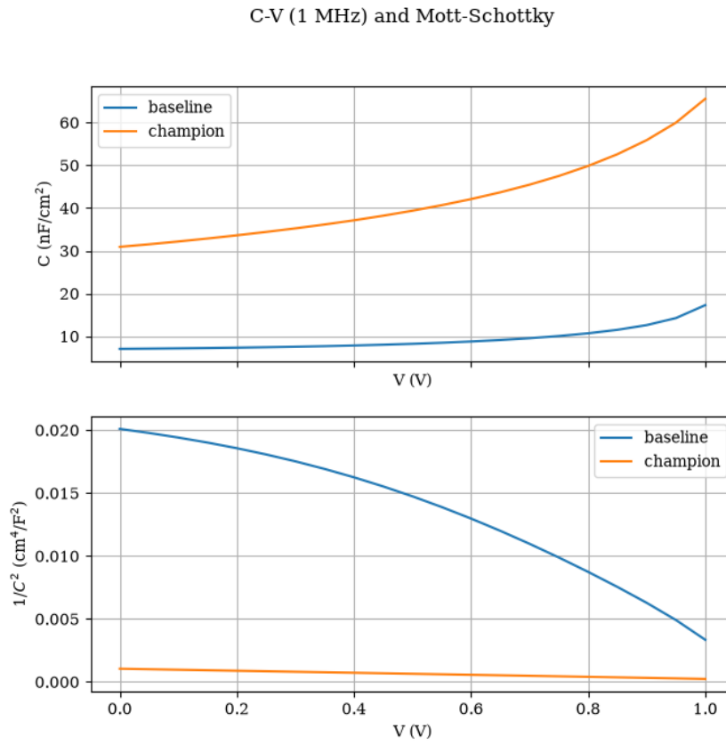
Figure 6: Capacitance–voltage (1 MHz) and Mott–Schottky plots for baseline and champion.
