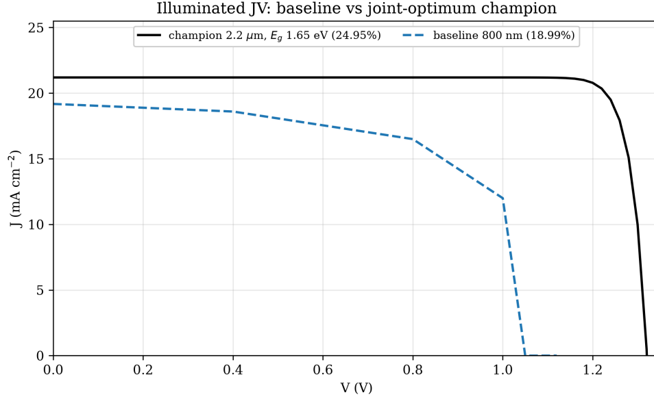
Figure 2: Illuminated current–voltage curves: baseline (800 nm, 18.99%) versus joint-optimum champion (2.2 \mu\text{m} , 24.95%).
