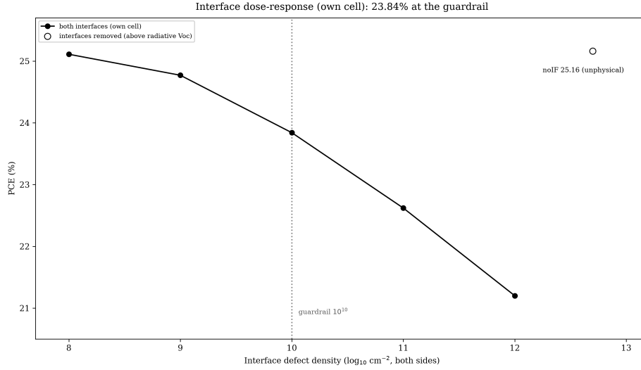
Figure 10: Same cell at graded interface quality: efficiency vs N_{if} (both sides). No literature scale bar is shown: cross-stack mapping is not claimed (Section 7.0).
