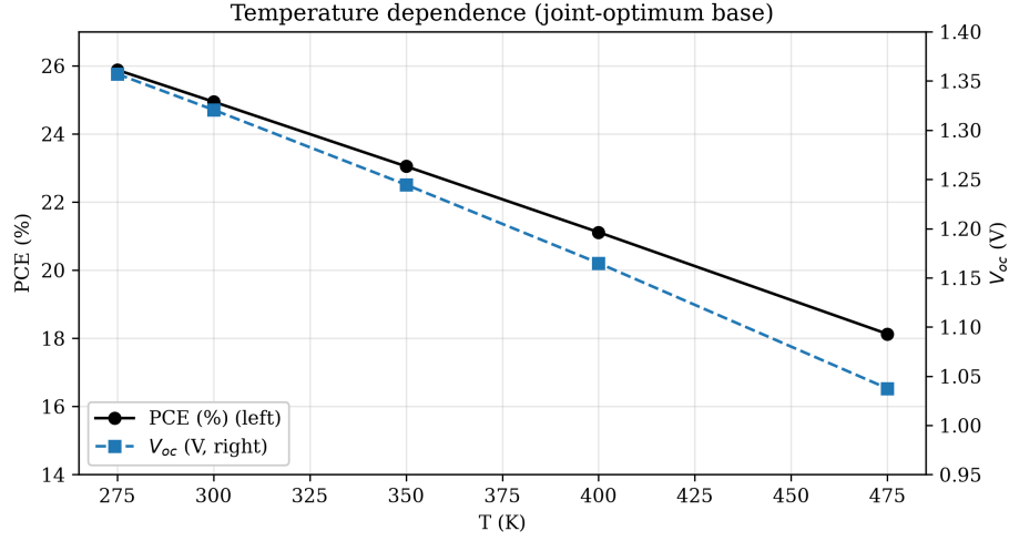
Figure 9: Efficiency and open-circuit voltage versus operating temperature at the joint-optimum base ( R_s = 0 ); the 475 K end is a solver stress test that ignores E_g(T) and black-phase stability.
