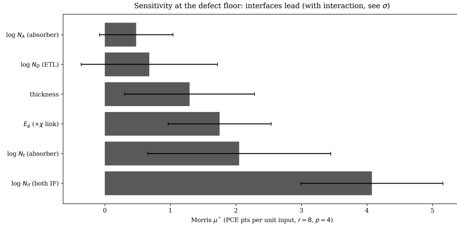
Figure 11: Morris \mu^* (bars) with interaction spread \sigma (whiskers). Ranking is regime-conditional: interfaces lead at the defect floor, bulk defects at routine levels (Table 15); large \sigma signals interactions.
