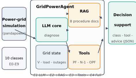
Fig. 2. Agent architecture.
