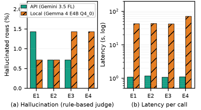
Fig. 5. Response-level any-tag hallucination (automated rule-based judge) and latency (log scale). Exact denominators in Table IV.
