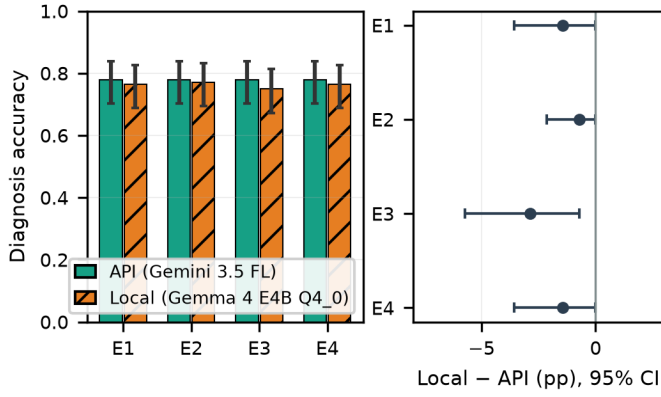
Fig. 3. (a) Diagnosis accuracy, local vs. API model, Wilson 95% CIs. (b) Paired diagnosis difference (Local - API) with bootstrap 95% CIs.
