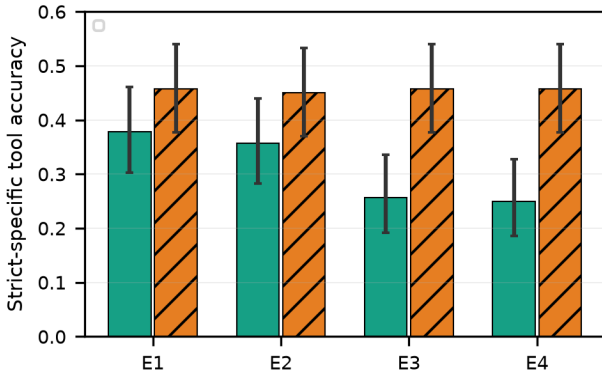
Fig. 4. Strict-specific tool-selection accuracy under the strict-specific metric (reference required set). Exact counts in Table V.
