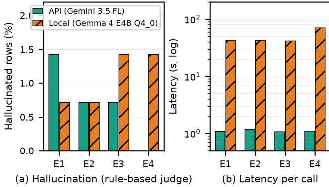
Fig. 5. Response-level any-tag hallucination (automated rule-based judge) and latency (log scale). Exact denominators in Table IV.
