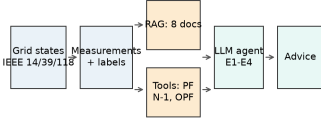
Fig. 2. Agent architecture.
