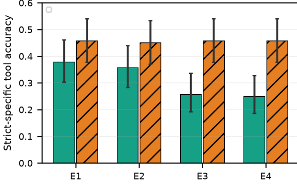
Fig. 4. Strict-specific tool-selection accuracy (reference required set). Exact counts in Tables IV and V.
