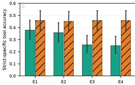
Fig. 4. Strict-specific tool-selection accuracy under the strict-specific metric (reference required set). Exact counts in Table ??.
