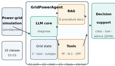
Fig. 2. Agent architecture.
