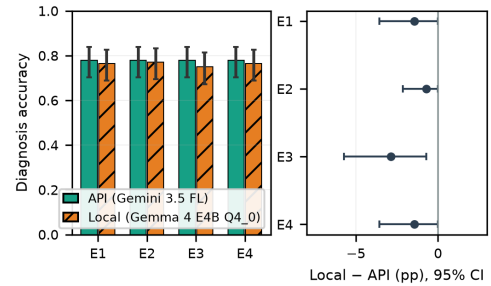
Fig. 3. (a) Diagnosis accuracy, local vs. API model, Wilson 95% CIs. (b) Paired diagnosis difference with bootstrap 95% CIs against reference margins (-10pp, -5pp).
