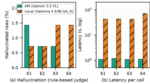
Fig. 5. Response-level any-tag hallucination (automated rule-based judge) and latency (log scale). Exact denominators in Table ??.
