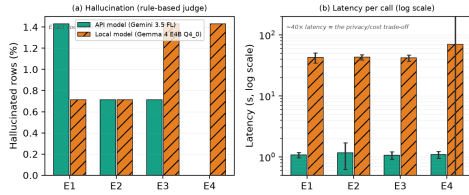
Fig. 5. Response-level any-tag hallucination (automated rule-based judge) and latency (log scale). Exact denominators in Table III.
