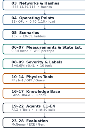
GridPowerAgent Pipeline (Stages 03-28)
