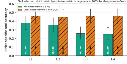
Fig. 4. Strict-specific tool-selection accuracy (reference required set). Exact counts in Table III.
