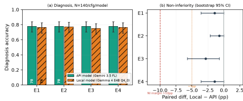
Fig. 3. (a) Diagnosis accuracy, local vs. API model, Wilson 95% CIs. (b) Paired diagnosis difference with bootstrap 95% CIs against reference margins ( -10\text{pp} , -5\text{pp} ).
