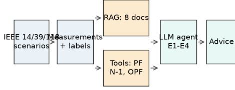
Fig. 2. Agent architecture.
