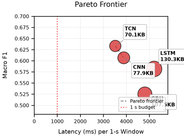
Fig. 4. Pareto: grouped CV macro vs. measured latency. TCN 3.61s (70.1KB) vs. CNN 3.79s (77.9KB) — TCN 5% faster; both RTF > 3 on ref kernels (red 1s line).
