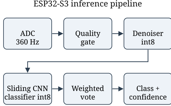
Fig. 2. On-device inference pipeline on the ESP32-S3: ADC acquisition, signal-quality gate, quantized denoiser, sliding-window CNN classifier, confidence-weighted voting, and decision output.
