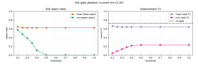
Fig. 6. SQI gate ablation: clean false-reject 62.6% at 0.35 (threshold 0.35, paper), corrupted reject 27.9%; downstream macro on kept clean 0.644 vs no-gate 0.728. Gate as tuned is not deployable without retuning.
