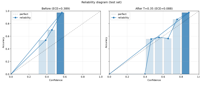
Fig. 3. Calibration reliability diagram on the held-out test set ( T = 0.350 , fit on val). ECE 0.389 \rightarrow 0.088, NLL 0.623 \rightarrow 0.244, Brier 0.323 \rightarrow 0.100.
