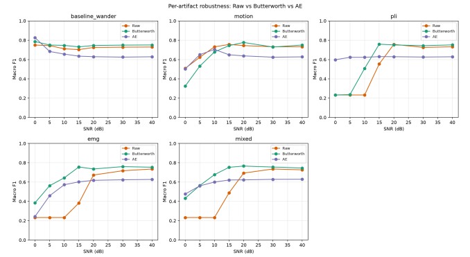
Fig. 5. Per-artifact robustness (5 types \times 7 SNR \times 3 front-ends). Butterworth wins 3/5 artifacts (BW, EMG, mixed), raw wins motion, AE only wins PLI low-SNR; denoiser cost 19 KB + 590 ms not justified.
