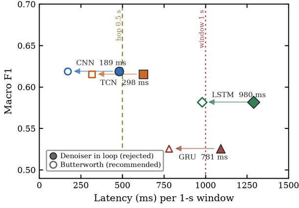
Fig. 5. Pareto: grouped CV macro vs. ESP-NN per-window latency. Filled = denoiser-in-loop (rejected); hollow + arrow = recommended Butterworth pipeline (classify+filter: 189/298 ms CNN/TCN, 980/781 ms LSTM/GRU). Bubble = flash size; colors/markers = architecture (legend). Budgets: 1-s window, 0.5-s hop.
