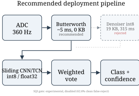
Fig. 2. Recommended deployment pipeline: ADC \rightarrow Butterworth ( \sim 5 ms, 0 KB) \rightarrow sliding CNN/TCN \rightarrow weighted vote. SQI gate and learned denoiser are evaluated but rejected.
