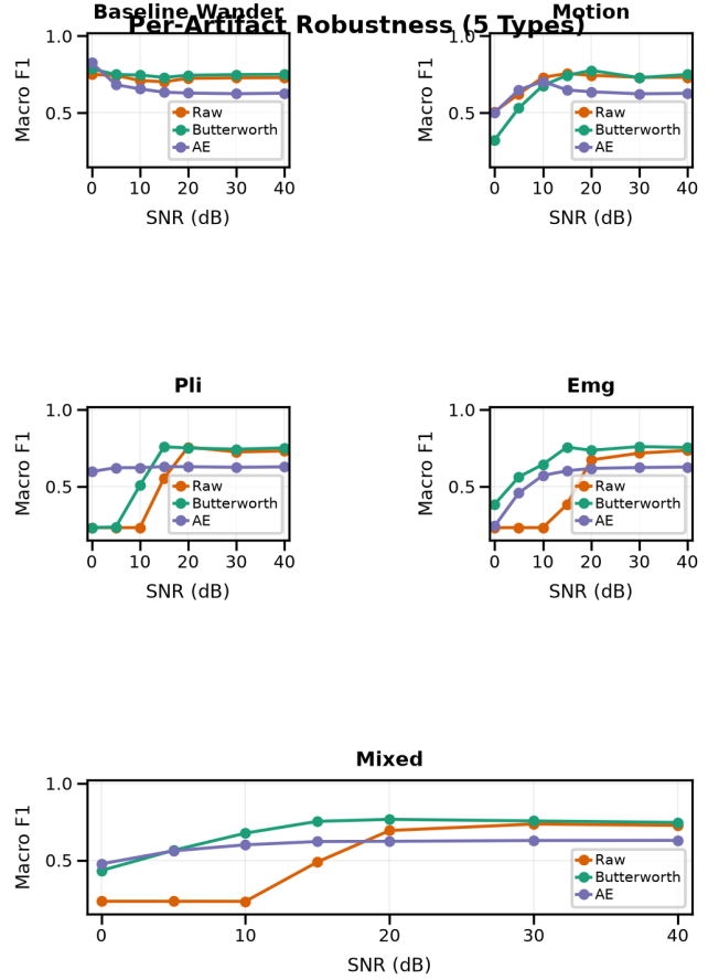
Fig. 5. Per-artifact robustness (5 types \times 7 SNR, single-column 3 rows: 2+2+1). Butterworth wins 3/5, raw wins motion, AE only wins PLI low-SNR — denoiser not justified.
