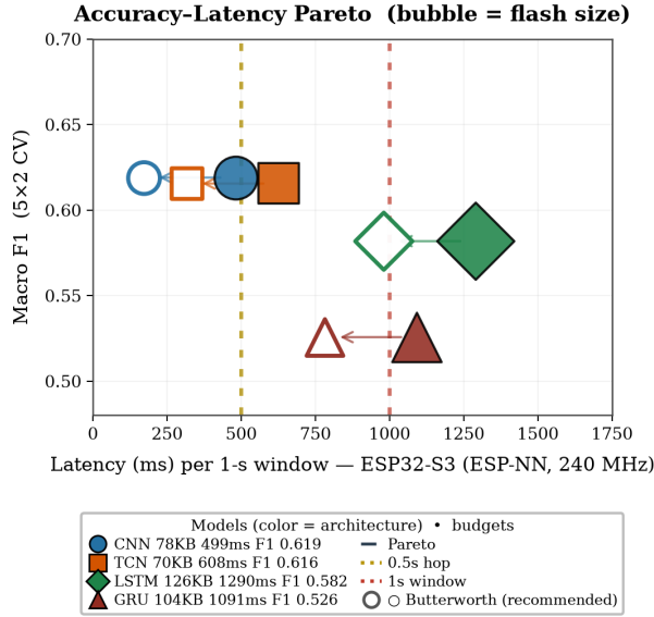
Fig. 5. Pareto: grouped CV macro vs. ESP-NN per-window latency. Filled = denoiser-in-loop (rejected); hollow + arrow = recommended Butterworth pipeline (classify+filter: 189/298 ms CNN/TCN, 980/781 ms LSTM/GRU). Bubble = flash size; colors/markers = architecture (legend). Budgets: 1-s window, 0.5-s hop.
