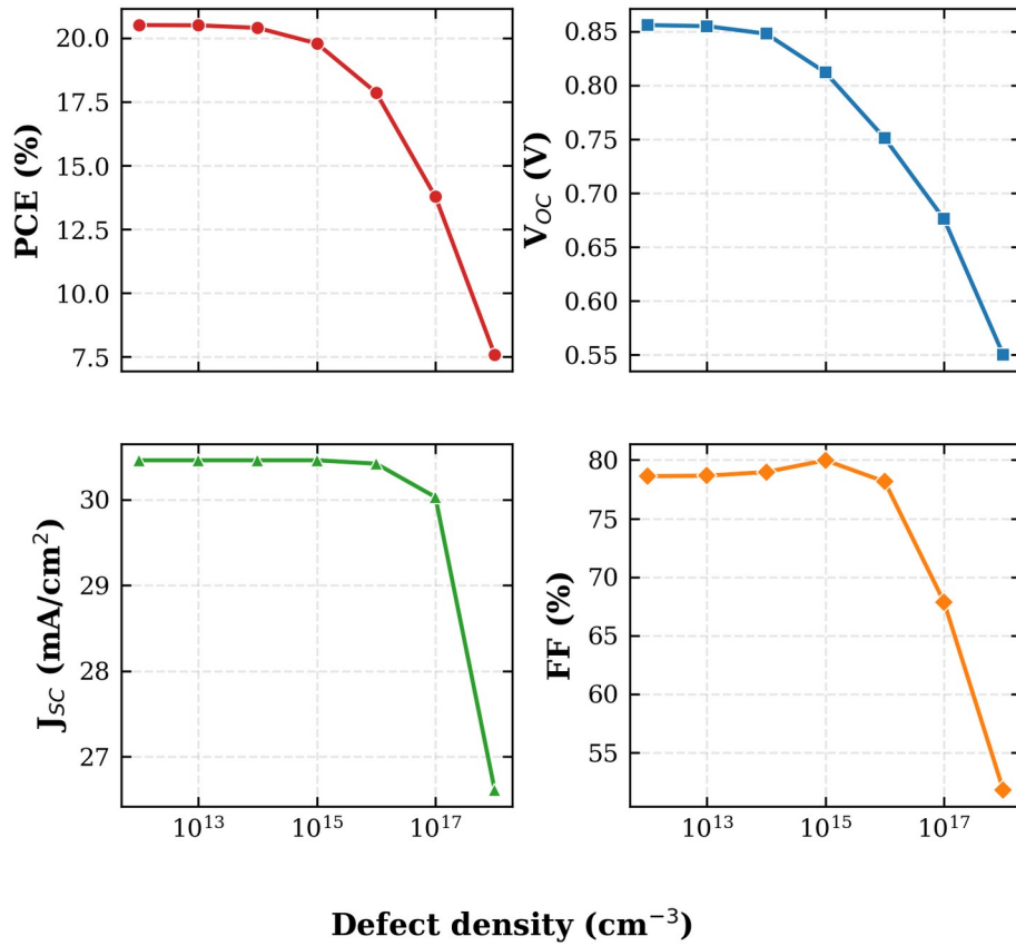
FIG. 4. Variation of PCE, V_{OC} , J_{SC} , and FF with RbGeI 3 absorber defect density. The device is essentially insensitive to defect densities below 10^{15} cm -3 but degrades sharply at higher values due to SRH recombination.
