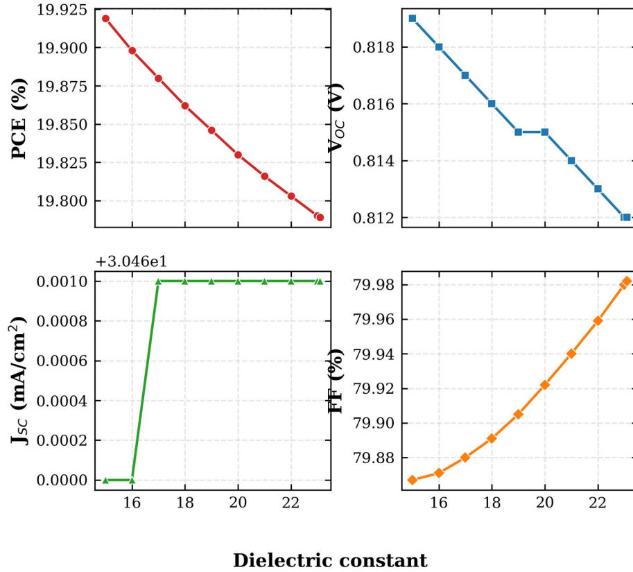
FIG. 5. Variation of PCE, V_{OC} , J_{SC} , and FF with the RbGeI 3 absorber dielectric constant. The effect is small within the studied range, with lower \epsilon_r values being slightly more favourable.
