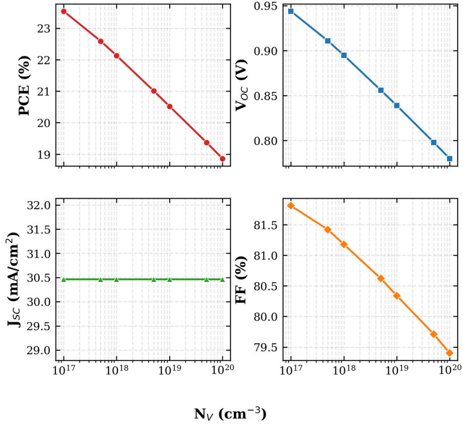
FIG. 13. Variation of PCE, V_{OC} , J_{SC} , and FF with the valence-band effective density of states N_V . The effect is more pronounced than for N_C .
