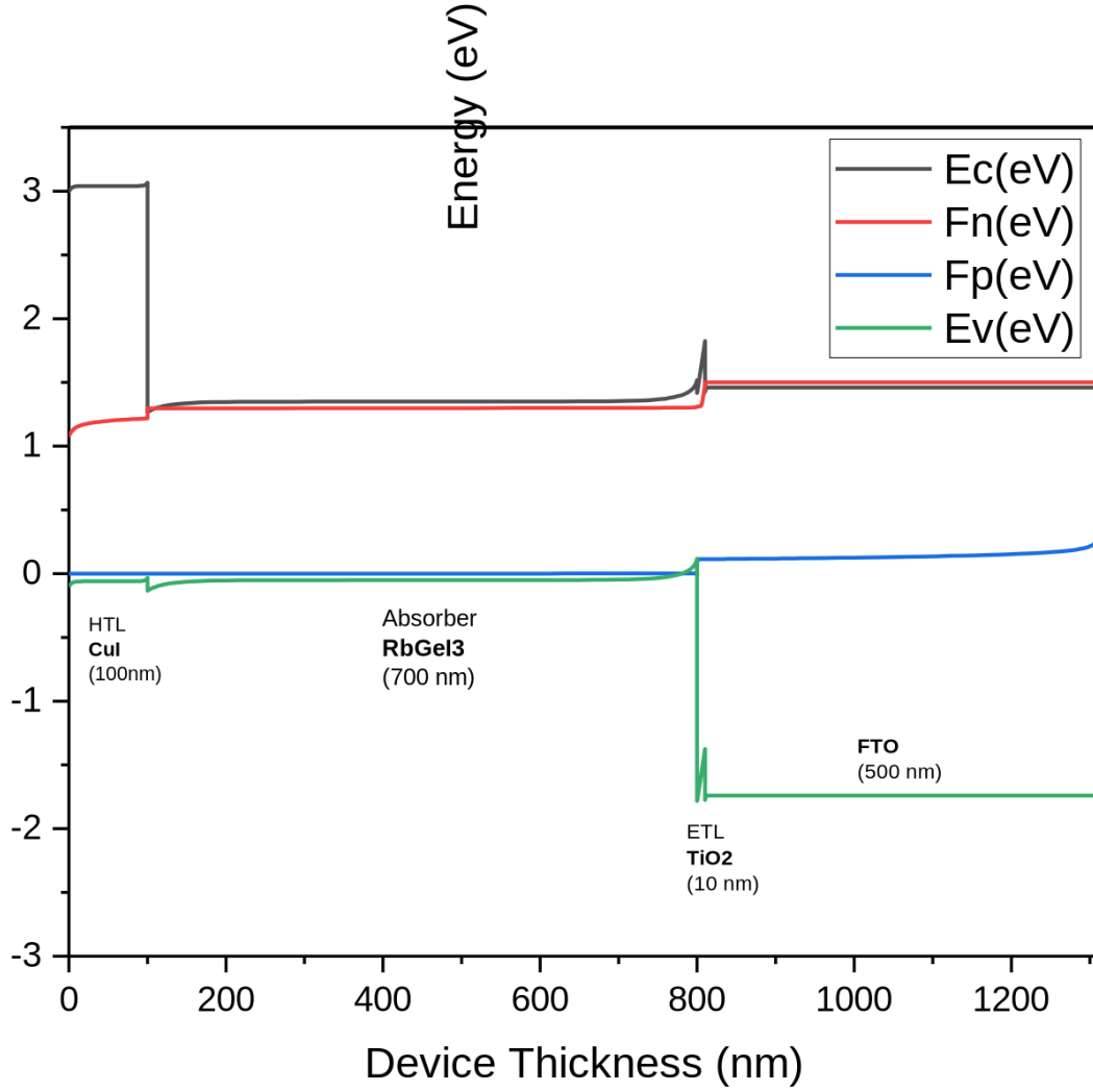
FIG. 15. Equilibrium energy band diagram of the optimized CuI/RbGeI 3 /TiO 2 /FTO solar cell, showing the conduction-band edge ( E_c ), valence-band edge ( E_v ), and quasi-Fermi levels ( F_n , F_p ) across the device stack.
