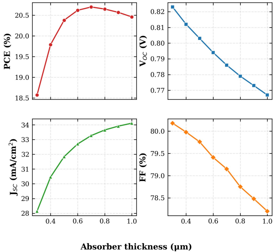
FIG. 3. Variation of PCE, V OC , J SC , and FF with RbGeI 3 absorber thickness. The PCE peaks at 0.7 \mu\text{m} , beyond which recombination losses offset the gain in optical absorption.
