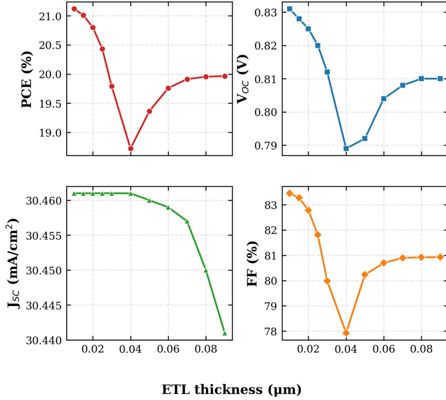
FIG. 10. Variation of PCE, V OC , J SC , and FF with the TiO 2 ETL thickness. The PCE is highest at the thinnest ETL (10 nm), reflecting the shorter electron transport path.
