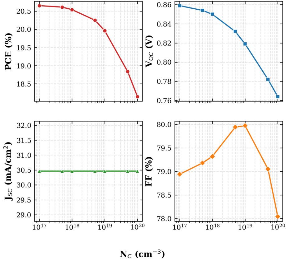
FIG. 12. Variation of PCE, V_{OC} , J_{SC} , and FF with the conduction-band effective density of states N_C .
