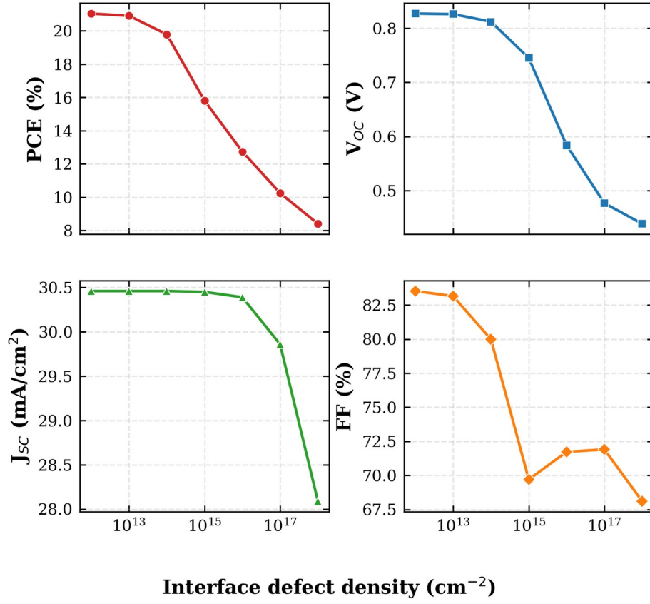
FIG. 7. Variation of PCE, V_{OC} , J_{SC} , and FF with the \text{TiO}_2/\text{RbGeI}_3 interfacial defect density. Performance degrades sharply above 10^{14} \text{ cm}^{-2} , indicating high sensitivity to absorber/ETL interface quality.
