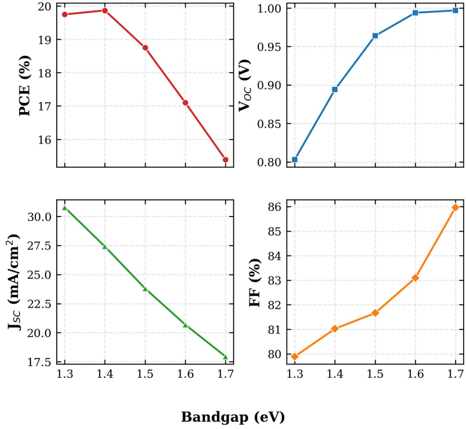
FIG. 9. Variation of PCE, V_{OC} , J_{SC} , and FF with the RbGeI_3 absorber bandgap. The PCE peaks at 1.4 eV, close to the Shockley–Queisser optimum for a single-junction cell.
