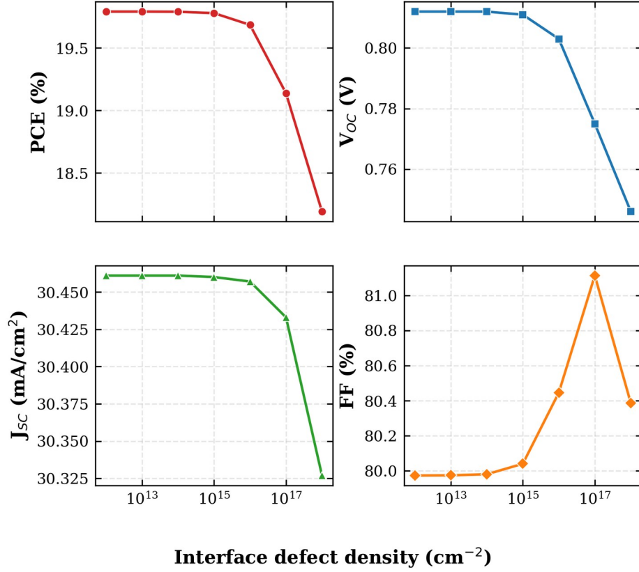
FIG. 8. Variation of PCE, V_{OC} , J_{SC} , and FF with the RbGeI 3 /CuI interfacial defect density. The HTL/absorber interface is markedly more tolerant than the absorber/ETL interface, thanks to the large conduction-band offset at the CuI/RbGeI 3 junction.
