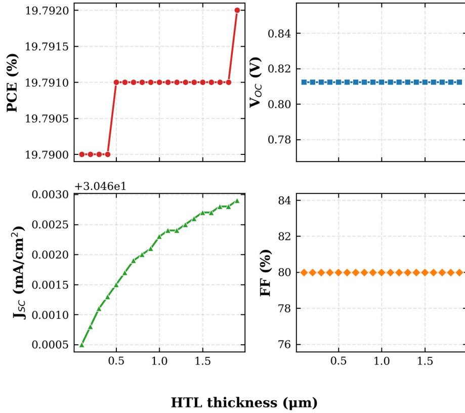
FIG. 11. Variation of PCE, V_{OC} , J_{SC} , and FF with the CuI HTL thickness. The HTL thickness has negligible influence on device performance.
