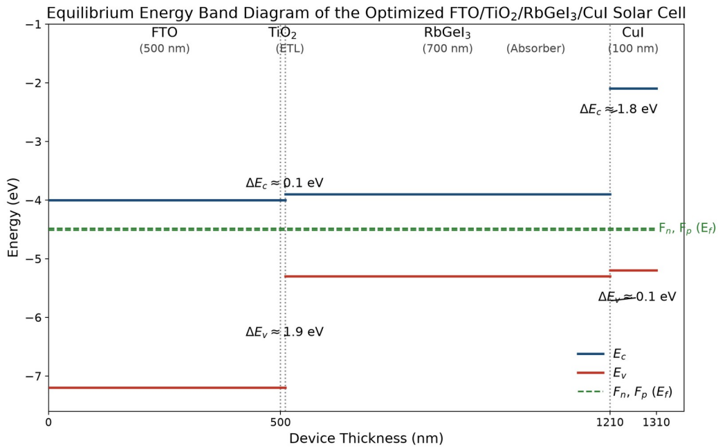
Fig. 15. Equilibrium energy band diagram of the optimized CuI/RbGeI 3 /TiO 2 /FTO solar cell, showing the conduction-band edge ( E_c , blue) and valence-band edge ( E_v , red) across all four layers. The 1.8 eV conduction-band offset at CuI/RbGeI 3 blocks electron back-transfer, while the 0.10 eV conduction-band step at RbGeI 3 /TiO 2 supports efficient electron extraction.
