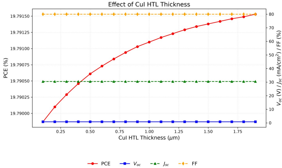
Fig. 11. Variation of PCE, V_{\text{OC}} , J_{\text{SC}} , and FF with CuI HTL thickness. The performance is essentially independent of HTL thickness; 100 nm is retained to minimise material usage.
