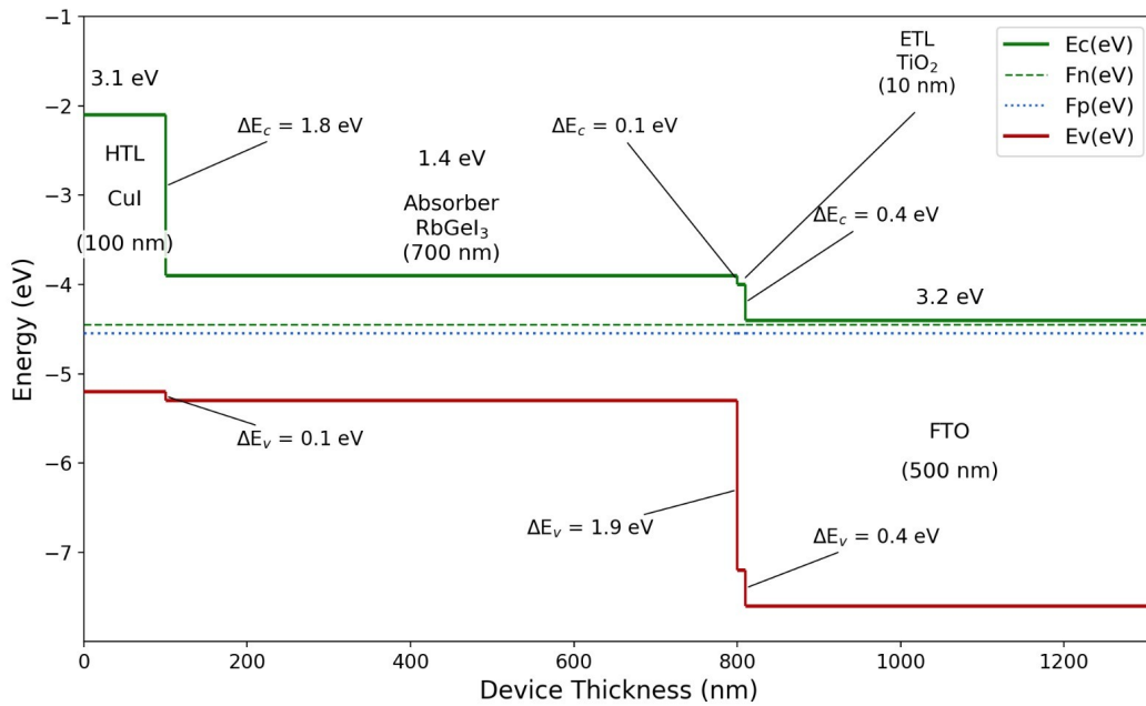
Fig. 15. Energy band diagram of the optimized FTO/TiO 2 /RbGeI 3 /CuI/Au solar cell under illumination, showing the conduction-band edge ( E_c ), valence-band edge ( E_v ), electron quasi-Fermi level ( F_n ), and hole quasi-Fermi level ( F_p ). The 1.8 eV conduction-band offset at the CuI/RbGeI 3 interface suppresses electron back-transfer, while the 0.10 eV conduction-band offset at the RbGeI 3 /TiO 2 interface facilitates electron extraction. The 1.90 eV valence-band offset at the RbGeI 3 /TiO 2 interface provides an energetic barrier against hole injection into TiO 2 .
