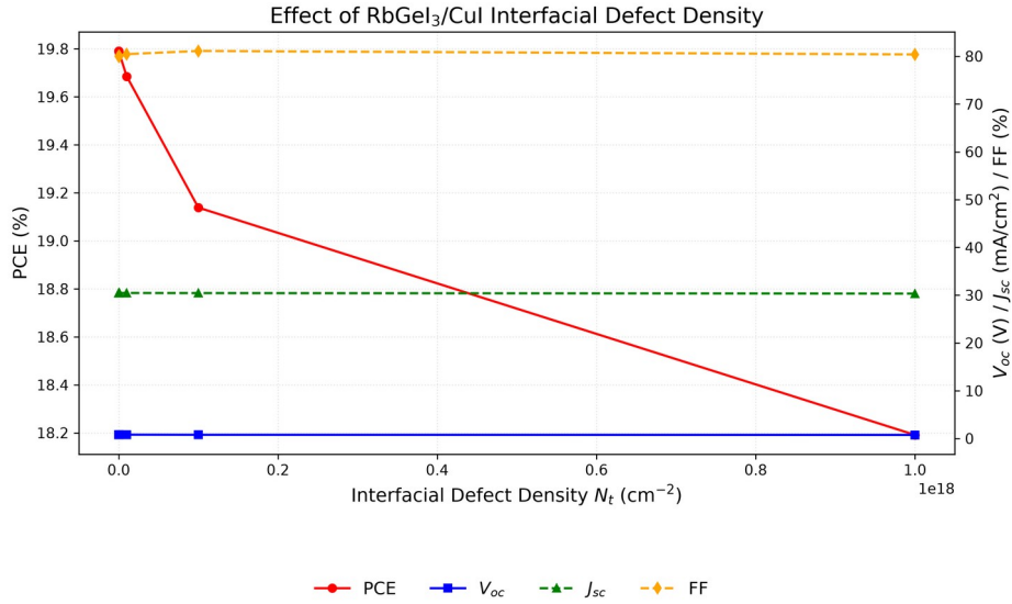
Fig. 8. Variation of PCE, V_{oc} , J_{sc} , and FF with RbGeI 3 /CuI interfacial defect density. The interface is markedly more defect-tolerant than the TiO 2 /RbGeI 3 interface; 10^{14} cm -2 is retained.
