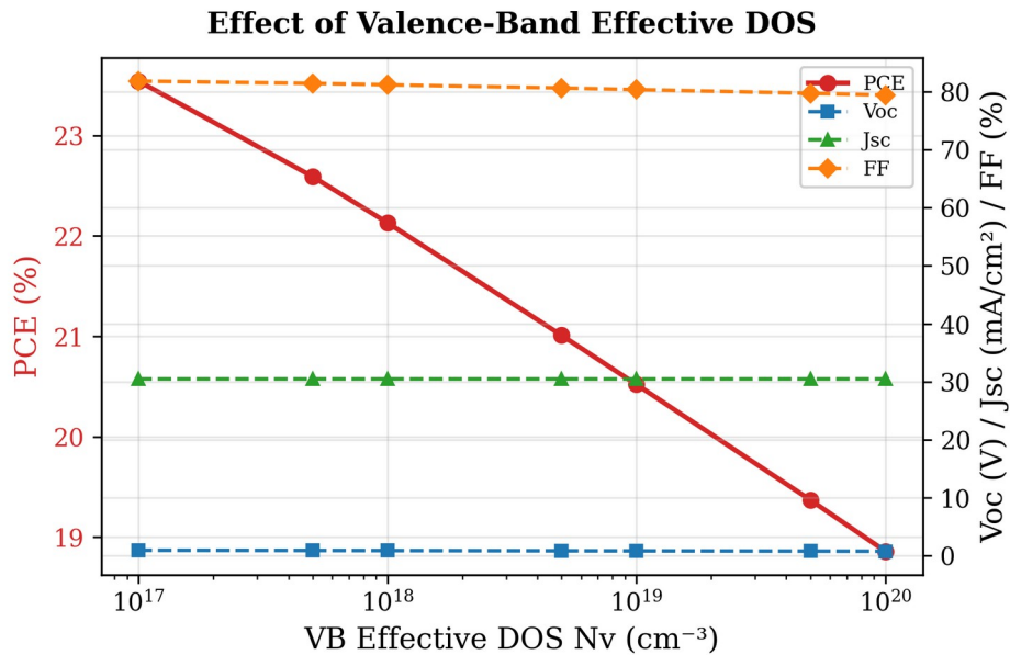
Fig. 13. Variation of PCE, V_{oc} , J_{sc} , and FF with valence-band effective density of states N_v . The effect is more pronounced than for N_c ; the best value of 10^{17} \text{ cm}^{-3} is retained.
