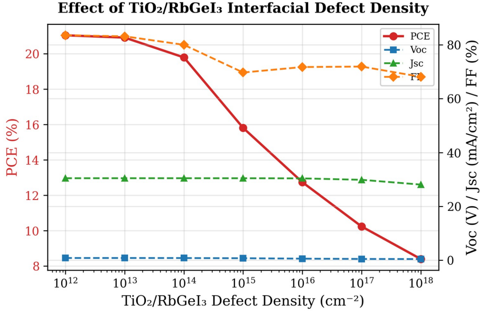
Fig. 7. Variation of PCE, V_{oc} , J_{sc} , and FF with TiO 2 /RbGeI 3 interfacial defect density. Performance degrades sharply above 10 14 cm -2 . The RbGeI 3 /CuI interface (Section V.G) was also evaluated and found to be significantly more defect-tolerant: PCE decreased only from 19.79% to 18.19% as defect density increased from 10 12 to 10 18 cm -2 , confirming that the TiO 2 /RbGeI 3 interface is the performance-limiting heterojunction in this device.
