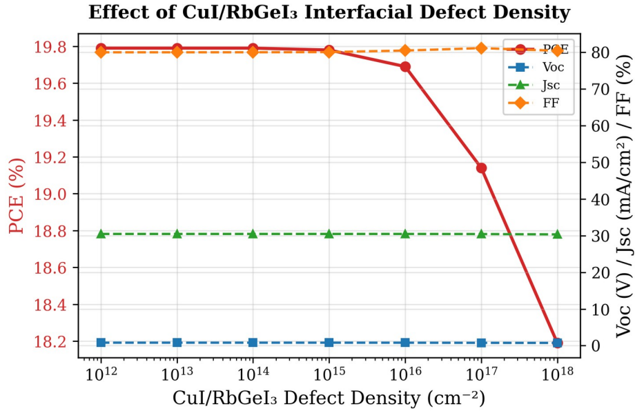
Fig. 8. Variation of PCE, V_{oc} , J_{sc} , and FF with RbGeI 3 /CuI interfacial defect density. The interface is markedly more defect-tolerant than the TiO 2 /RbGeI 3 interface; 10^{14} \text{ cm}^{-2} is retained.
