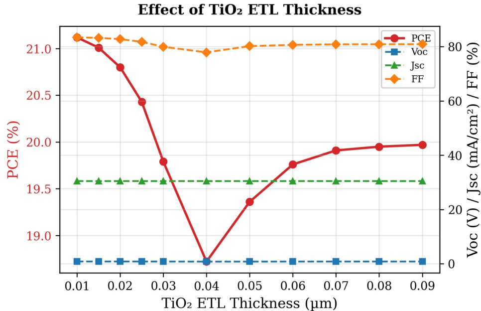
Fig. 10. Variation of PCE, V_{oc} , J_{sc} , and FF with TiO 2 ETL thickness. PCE is highest at the thinnest ETL (10 nm), reflecting the shorter electron transport path.
