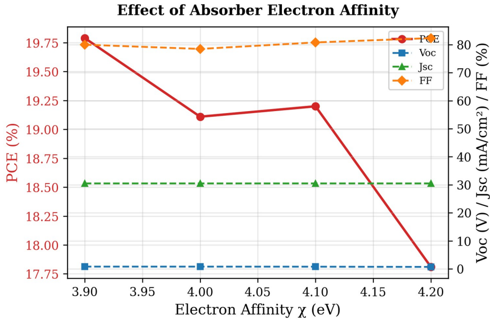
Fig. 6. Variation of PCE, V_{oc} , J_{sc} , and FF with RbGeI 3 absorber electron affinity. PCE is highest at \chi = 3.9 eV due to optimal band alignment with TiO 2 .
