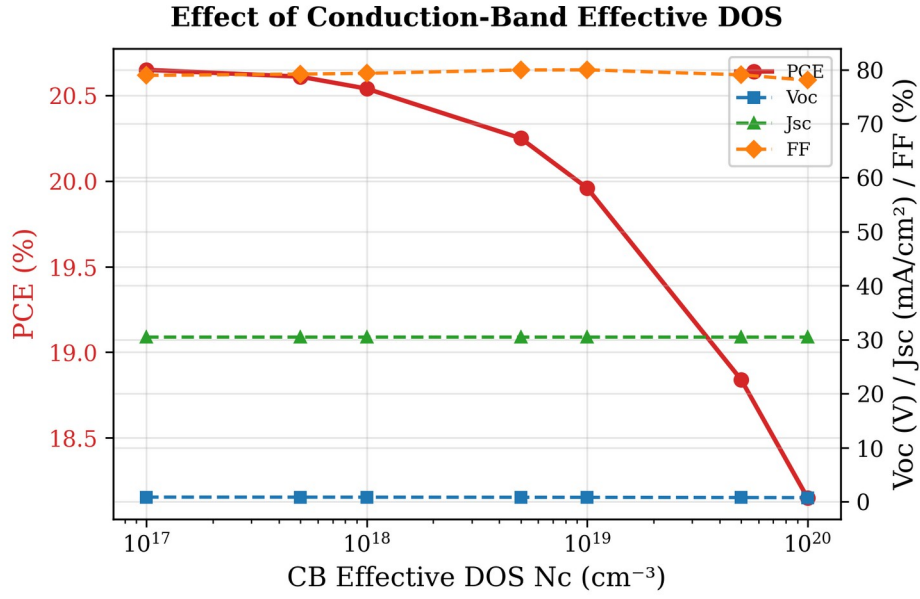
Fig. 12. Variation of PCE, V_{oc} , J_{sc} , and FF with conduction-band effective density of states N_c . Lower N_c is preferred; the best value of 10^{17} \text{ cm}^{-3} is retained.
