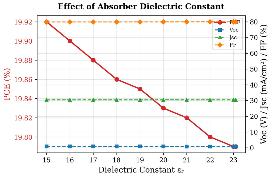
Fig. 5. Variation of PCE, V_{oc} , J_{sc} , and FF with RbGeI 3 absorber dielectric constant. The performance is essentially insensitive to \epsilon_r across the investigated range; \epsilon_r = 15 is retained.
