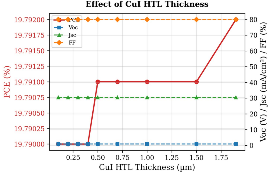
Fig. 11. Variation of PCE, V_{oc} , J_{sc} , and FF with CuI HTL thickness. The performance is essentially independent of HTL thickness; 100 nm is retained to minimise material usage.
