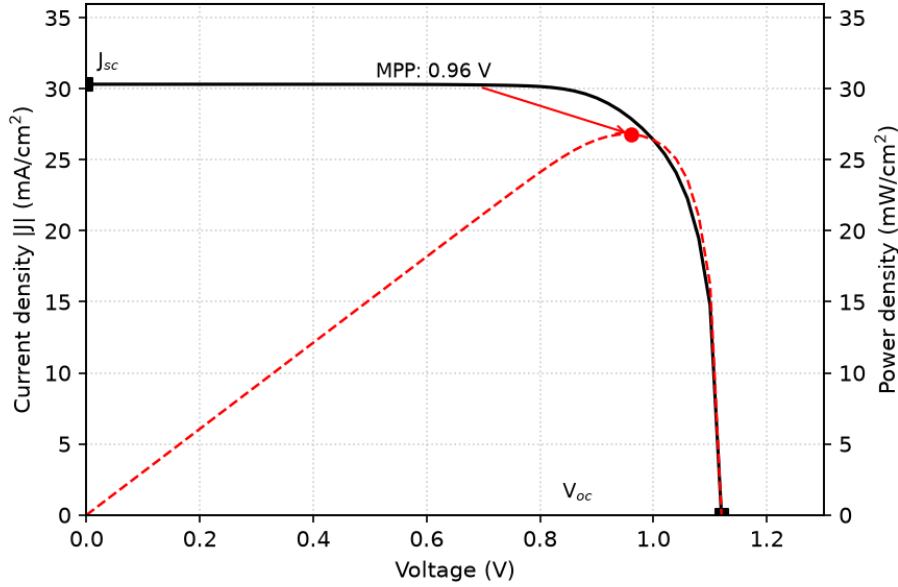
Fig. 16. Current density–voltage (J–V) curve of the optimized FTO/TiO 2 /RbGeI 3 /CuI/Au device under AM 1.5G illumination. The red dashed curve shows the output power density, with the maximum-power point marked.
