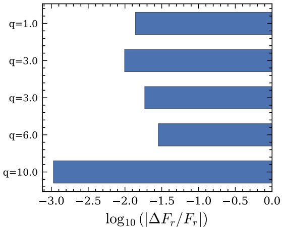
(a) F_r relative error
