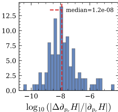
(e) \partial_{p_r} H (FD vs analytical)
