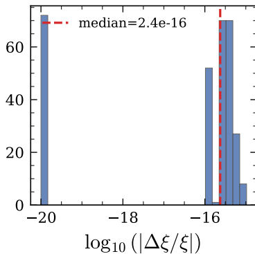
(e) \partial_{p_r} H (FD vs analytical)
