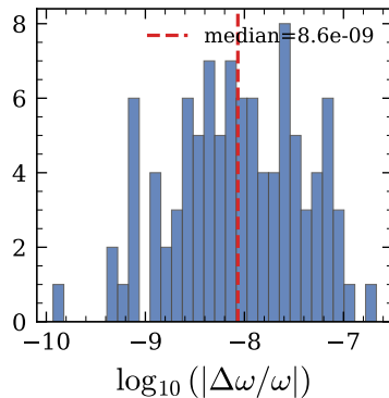
(f) \omega (FD vs analytical)
