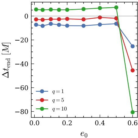
(a) Inspiral time offset
