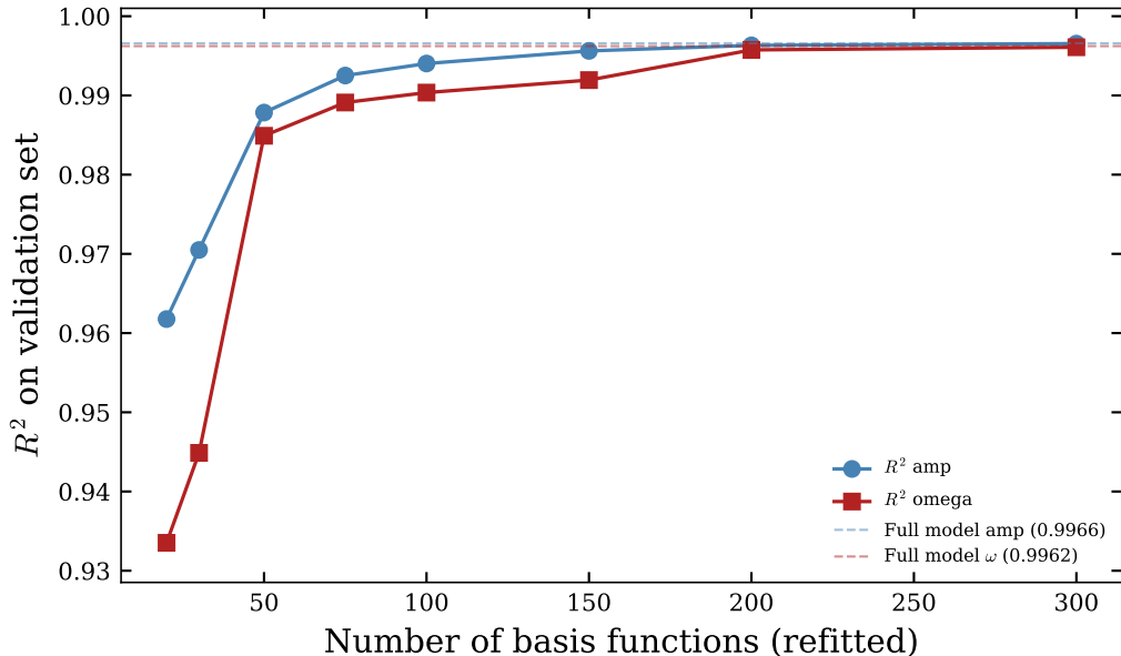
Skeleton Model Accuracy vs Number of Terms
