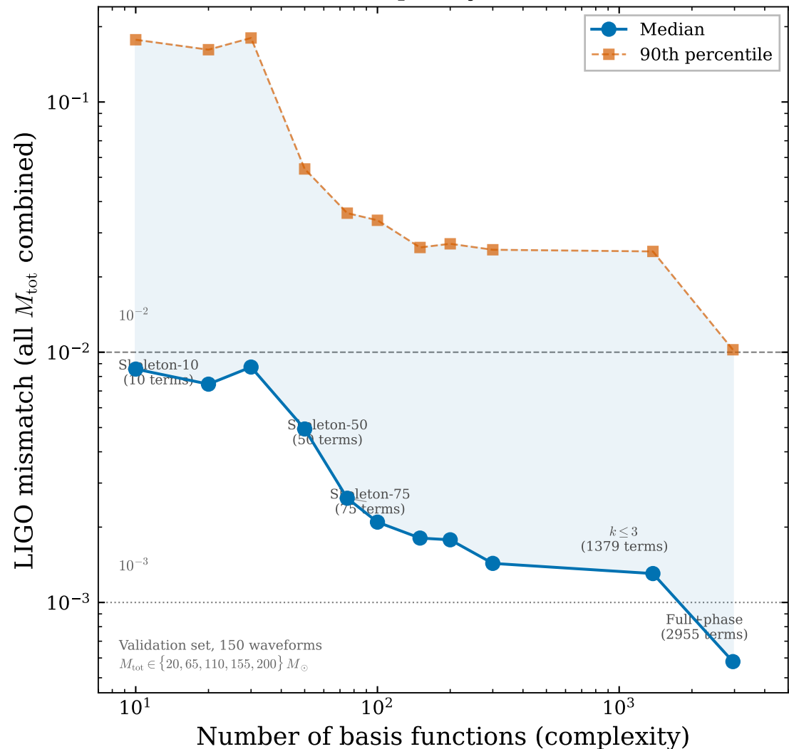
Pareto Front: Complexity vs LIGO Mismatch
