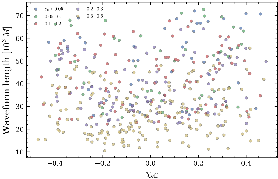
Length vs \chi_{\text{eff}} by eccentricity
