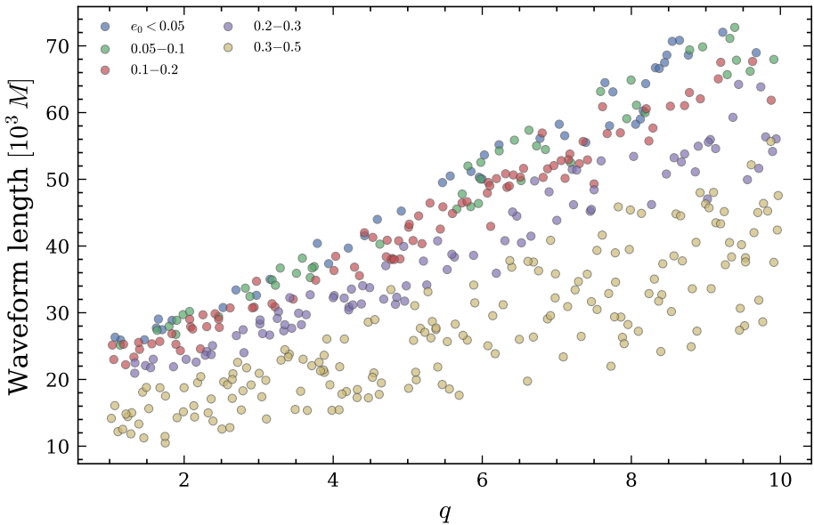
Length vs q by eccentricity
