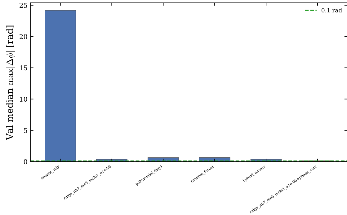
Dephasing progress
