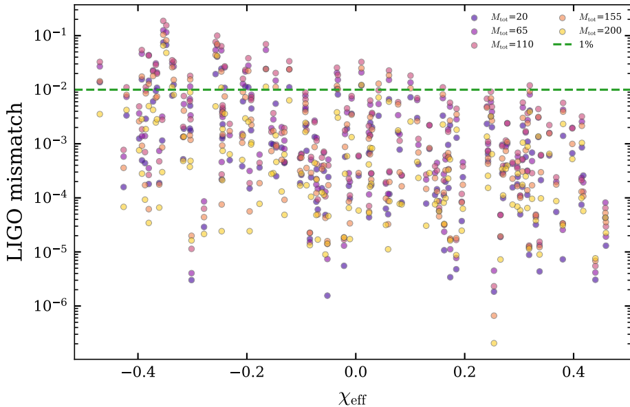
final_ridge_compactified_phase_corr: LIGO MM vs \chi_{\text{eff}}
