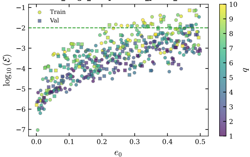
final_ridge_compactified_phase_corr
