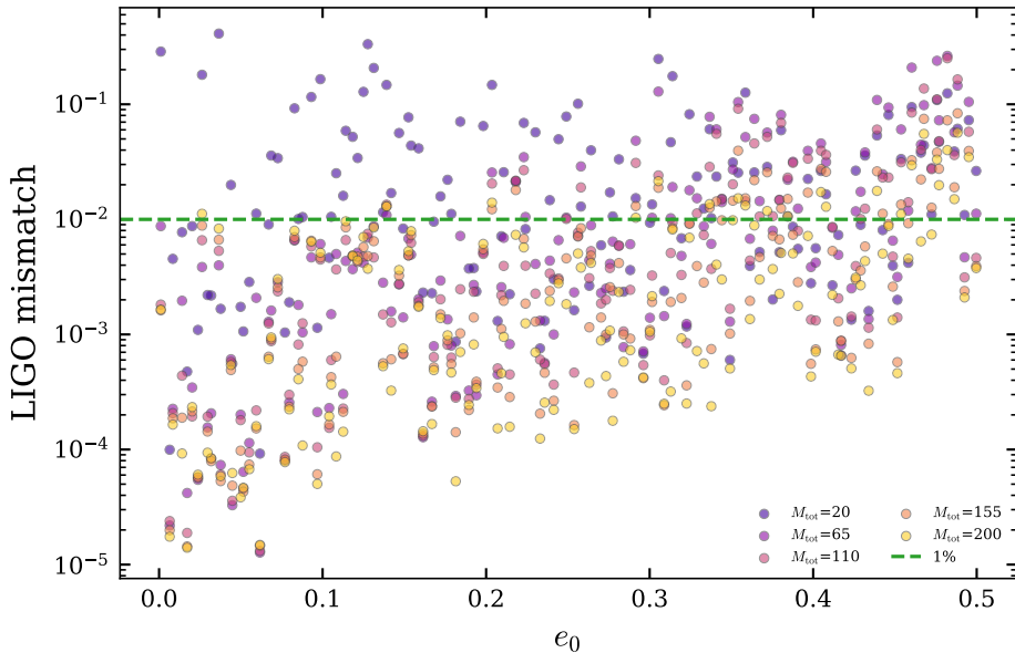
random_forest: LIGO MM vs e_0
