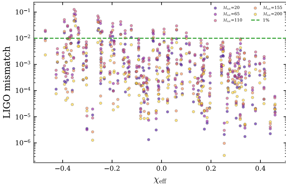
ridge_nh7_me5_mchi1_a1e-06+phase_corr: LIGO MM vs \chi_{\text{eff}}
