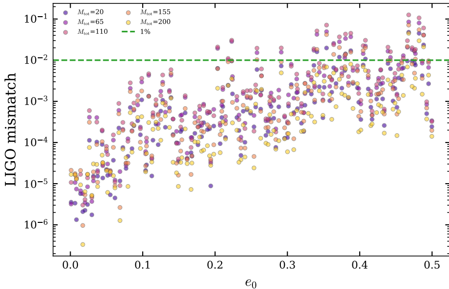
ridge_nh7_me5_mchi1_a1e-06+phase_corr: LIGO MM vs e_0
