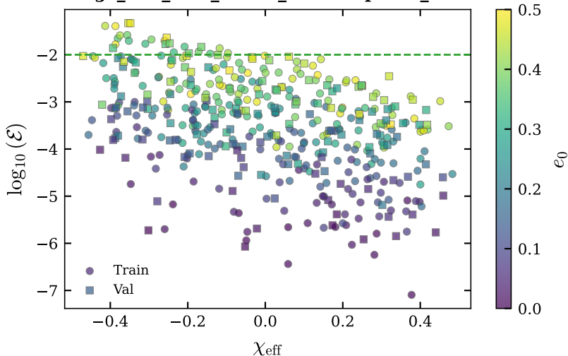
ridge_nh7_me5_mchi1_a1e-06+phase_corr
