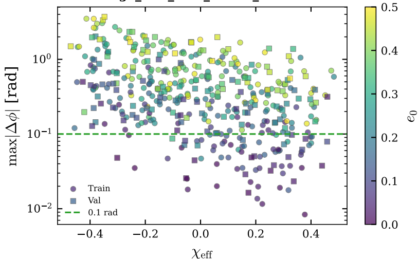
ridge_nh7_me5_mchi1_a1e-06
