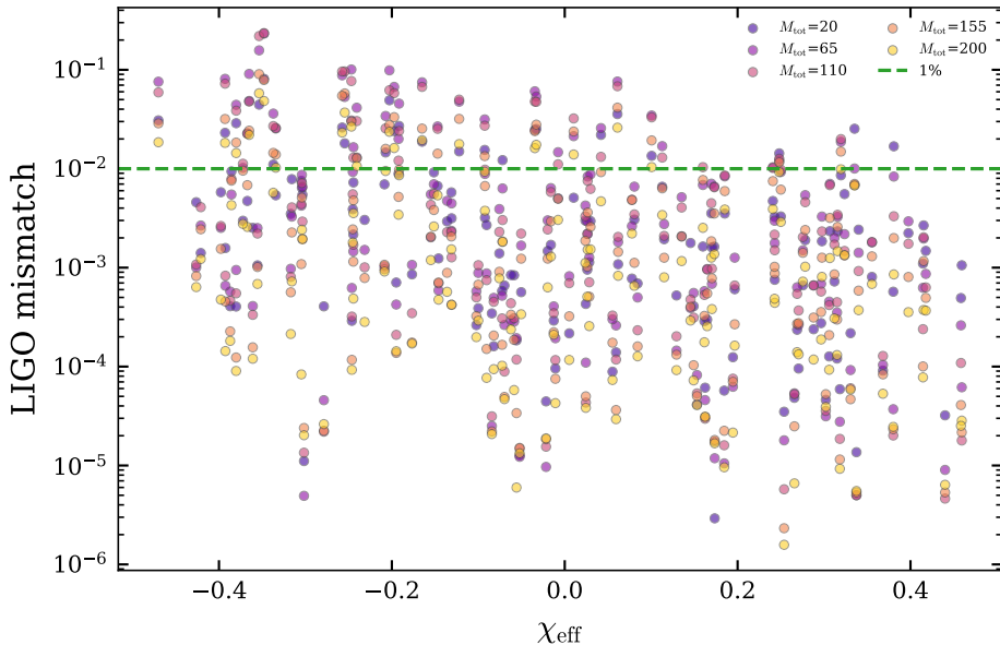
ridge_nh7_me5_mchi1_a1e-06: LIGO MM vs \chi_{\text{eff}}
