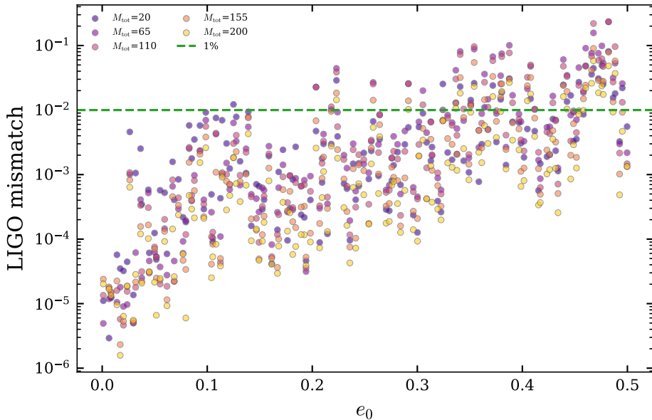
ridge_nh7_me5_mchi1_a1e-06: LIGO MM vs e_0
