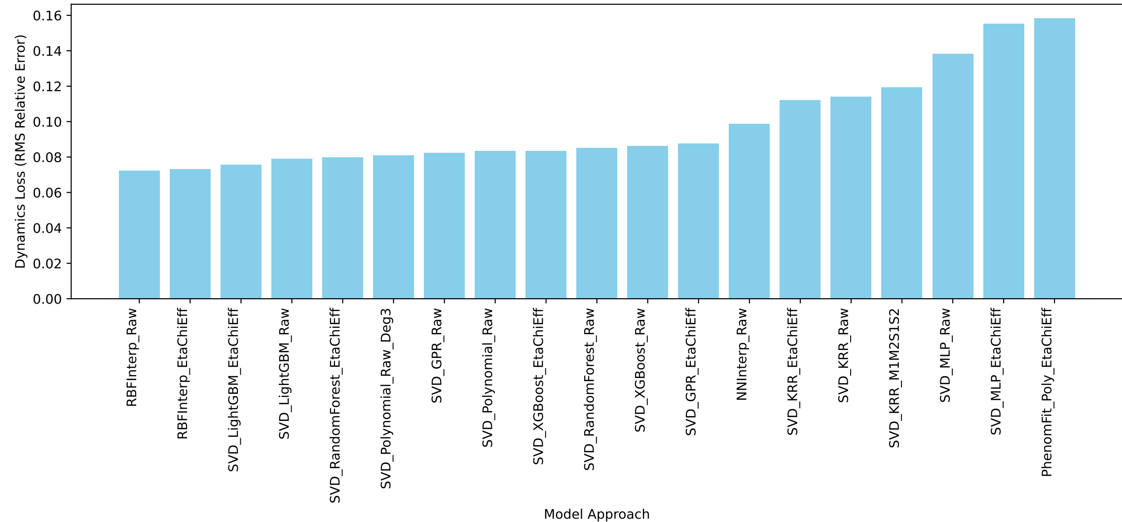
Loss Comparison for Dynamics Benchmark Models
