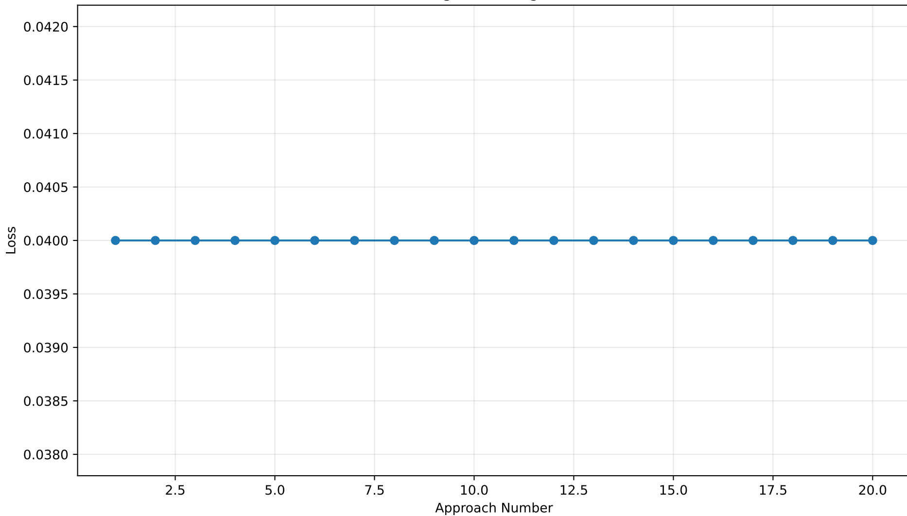
Ringdown: Progress
