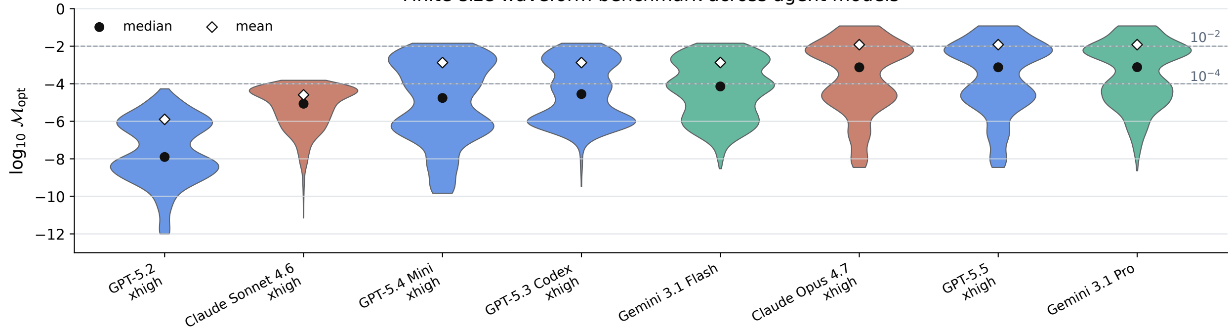
Finite-size waveform benchmark across agent models
