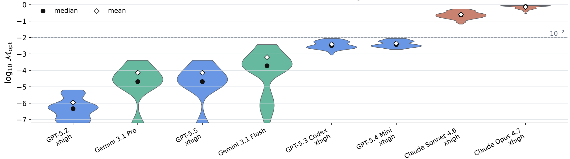
RG-tail waveform benchmark across agent models
