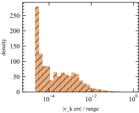
extratrees eff
