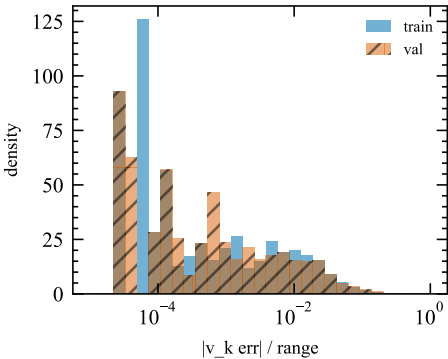
extratrees eff
