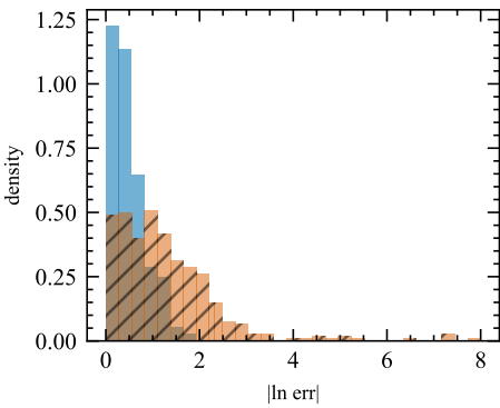
xgboost logq
