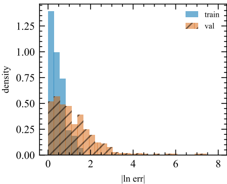
xgboost logq
