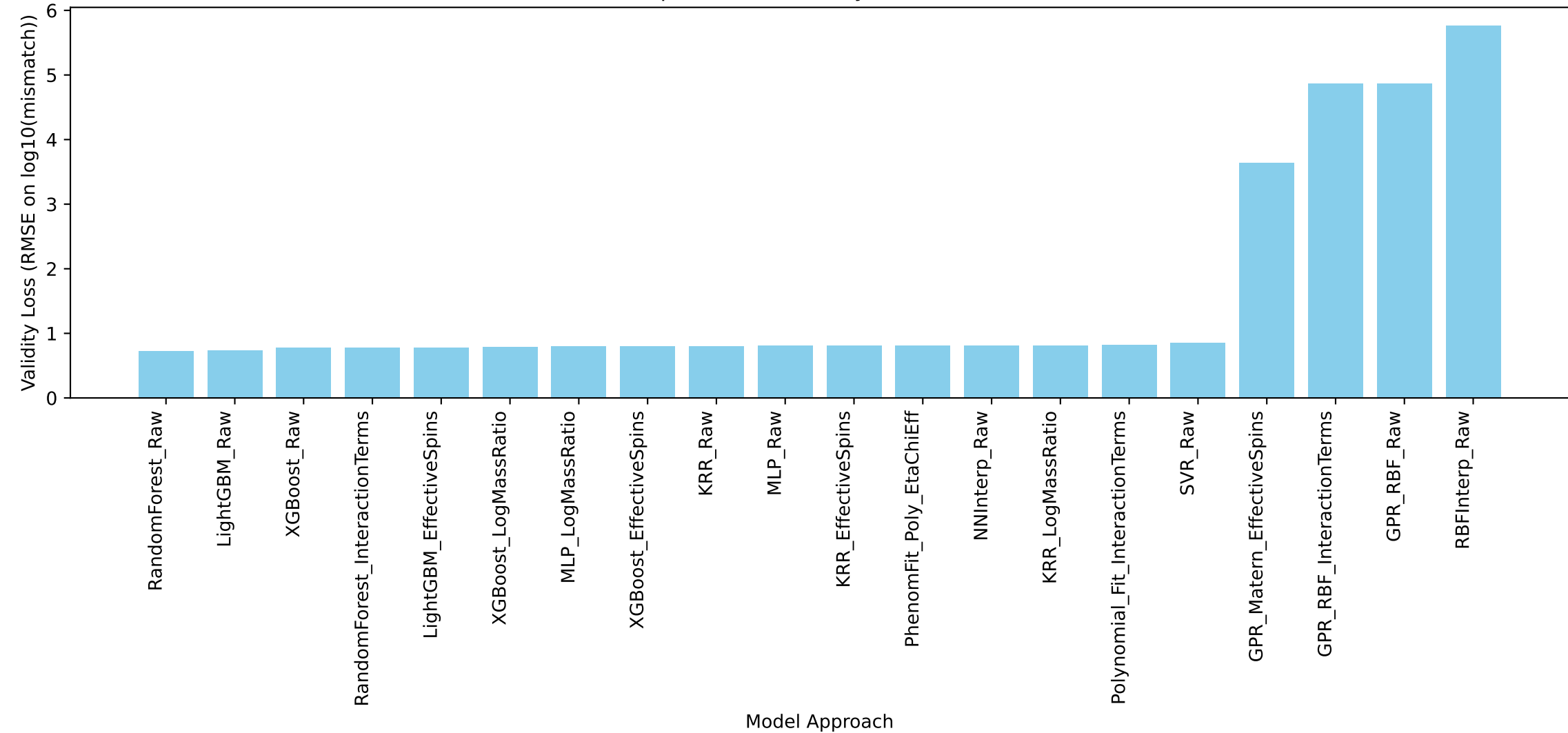
Loss Comparison for Validity Benchmark Models
