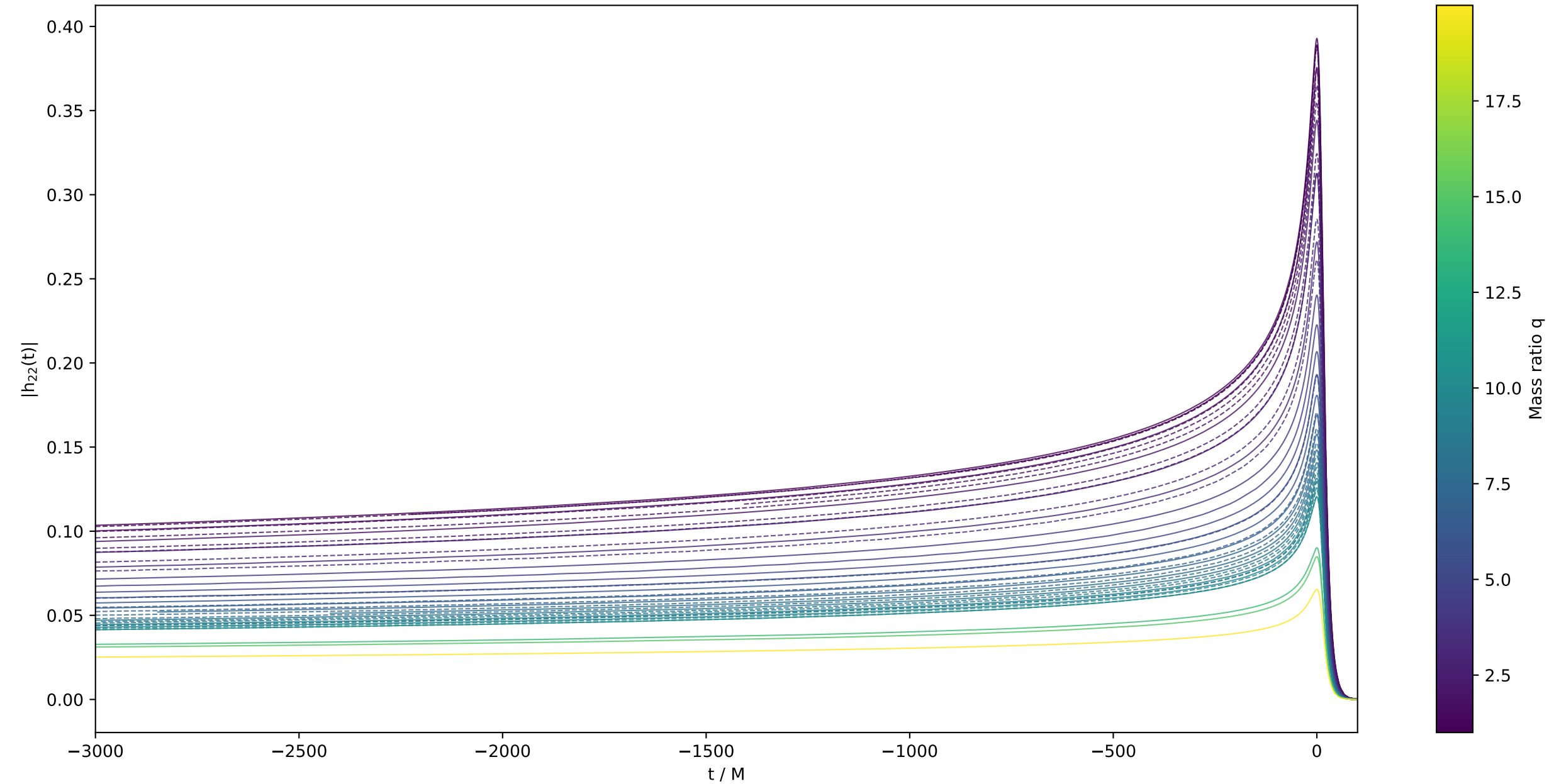
Analytic Bench: h_{22} Amplitudes (solid=train, dashed=val)
